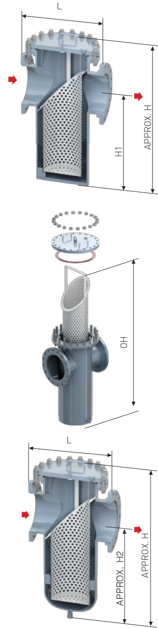
DIMENSION TABLE
