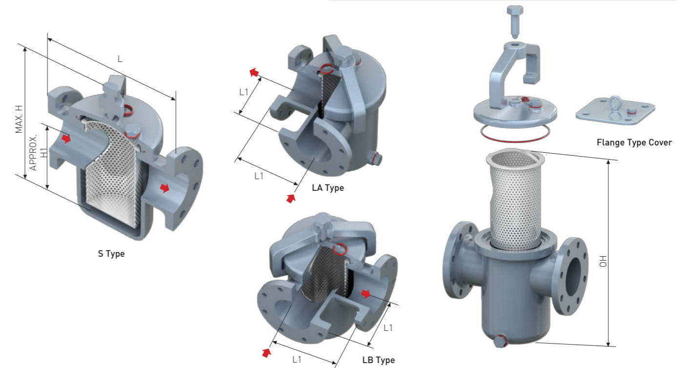
DIMENSION TABLE
